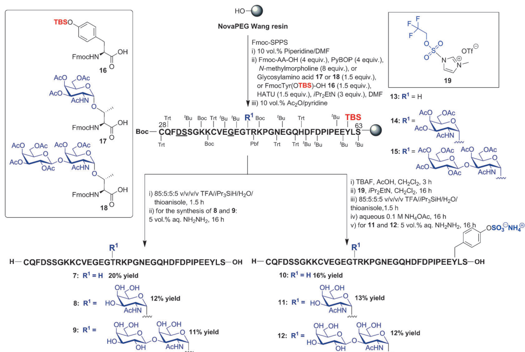
Scheme 1. Divergent solid-phase synthesis of differentially O -glycosylated and Tyr-sulfated HP6(28–63) fragments. TBS = tert -butyldimethylsilyl, Pbf = 2,2,4,6,7-pentamethyldihydrobenzofuran-5-sulfonyl, DS represents an Asp( t Bu)-Ser( \Psi^{\text{Me,Me}} pro) residue, G represents an N -(2,4-dimethoxybenzyl) Gly residue.
